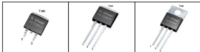
PG-TO263-3-2
